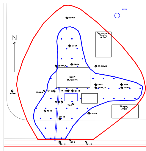
Injection Locations
