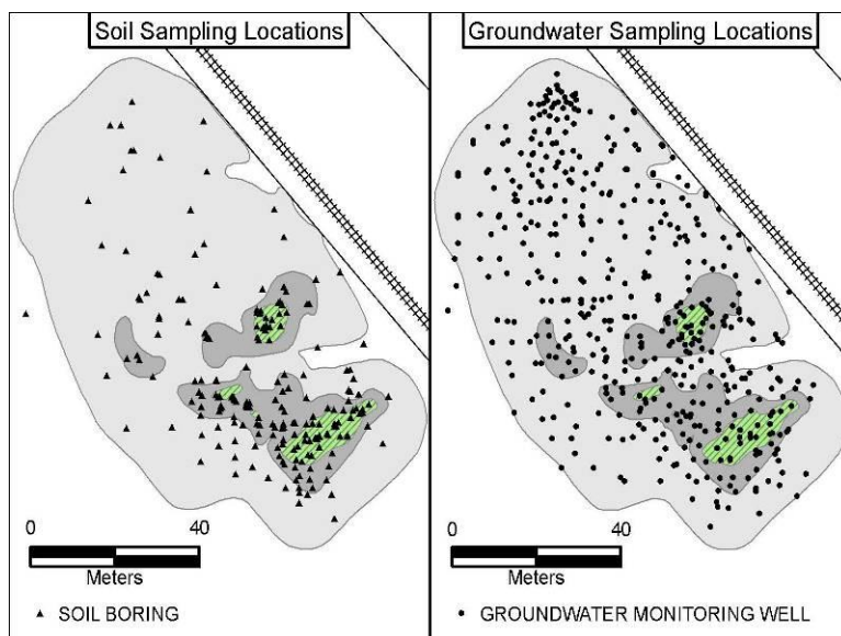
FIGURE 5. High-resolution data obtained from soil boring and groundwater well locations.
