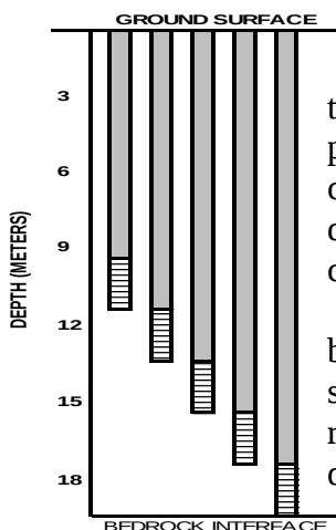
FIGURE 6. Nested wells.
