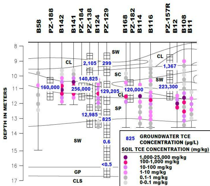
FIGURE 7. Typical cross section/transect.
