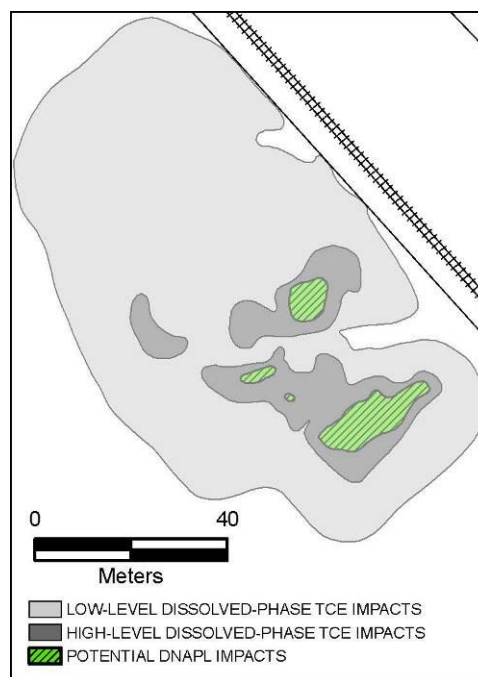
FIGURE 1. TCE plume.
